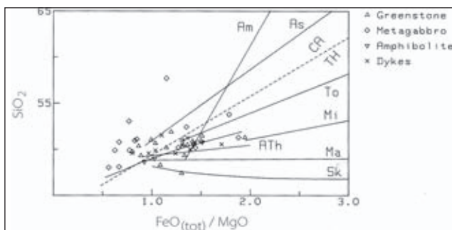
Fig. 28. All Váddás mafic rocks plotted on a \text{FeO}(\text{total})/\text{MgO} vs \text{SiO}_2 Diagram, showing a general evolutionary trend towards a tholeiitic composition – arc tholeiites or ocean-floor tholeiites. The spread of data points results largely from the presence of cumulate metagabbro samples. Trend lines after Miyashiro et al. (1982). CA = calc-alkaline, TH = tholeiitic, Am = Amagi volcano (Japan), To = Tofua Island (Tonga Arc), Mi = Miyake-jima (Izu-Bonin Arc), ATH = Abyssal tholeiite, Ma = Macaulay Island (Kermadec Arc), Unlabelled line = Kilauea (Hawaii).
