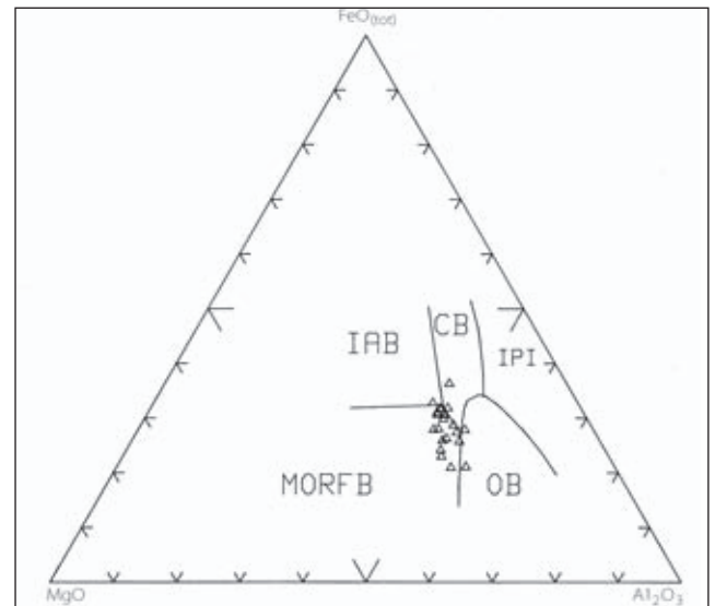
Fig. 30. Selected Váddás samples plotted on a \text{MgO}/\text{FeO}(\text{total})/\text{Al}_2\text{O}_3 diagram. MORFB = ocean-ridge and ocean-floor basalts, OB = orogenic basalt, IAB = ocean-island basalt, CB = continental basalt, IPI = spreading centre island basalt. Fields after Pearce et al. (1977).
