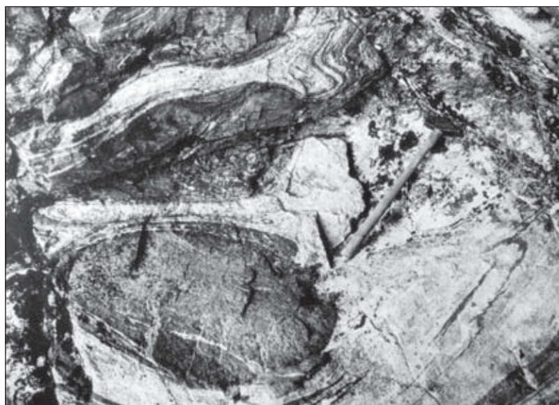
Fig. 24. Felsic pegmatitic intrusion in the Váddašgåissát Metagabbro. The gabbro fragments are subrounded and show flow banding. (Map reference UTM 523900–7740050, Nordreisa sheet, 1734.4, Photo I. Lindahl).
