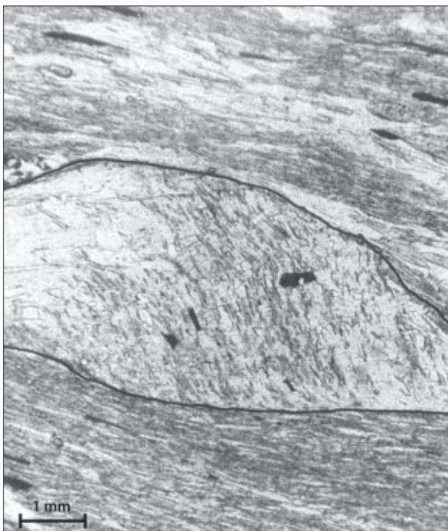
Fig. 4. Rotated, pre-tectonic, biotite porphyroblast from the Oksfjorrdalen Schist Member. The orientation of the inclusions is at a high angle to the schistosity. Plane-polarised light (sample VR 553, thin-section 7625, Photo I. Lindahl).
