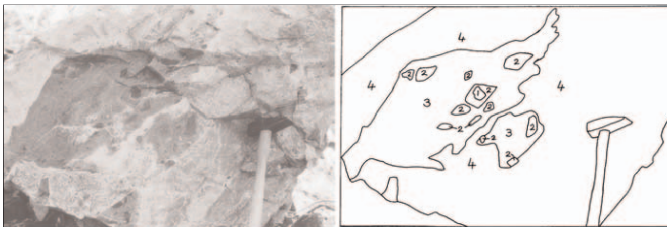
Fig. 25. Amphibole-bearing felsite containing blocks of more basic rocks. Apparent block-in-block textures may be due to reaction between felsic and mafic components. Loose boulder, Moskodalen. 1. Gabbroic rock with large mafic crystals – igneous texture; 2. Amphibolite or dolerite – granular texture; 3. Leucocratic amphibolite – granular texture; 4. Amphibole-bearing felsite with minor biotite-bearing pegmatite. (Map reference UTM 513150–7732200, Reisadalen sheet, 1734.3, Photo B. Stevens).
