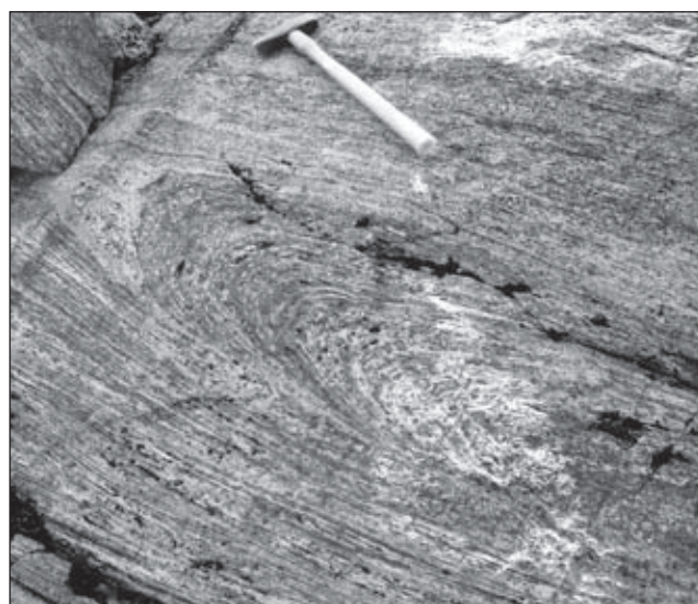
Fig. 19. Folded gneissosity in coarse- to very coarse-grained olivine-bearing Váddašgáissát Metagabbro. No obvious schistosity axial planar to the fold can be detected. (Map reference UTM 522200–7741700, Nordreisa sheet, 1734.4, Photo B. Stevens).
