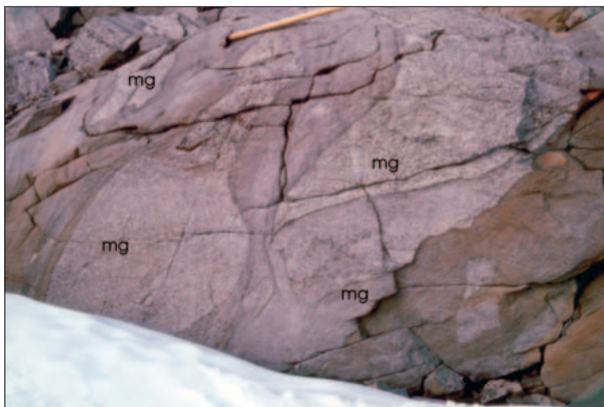
Fig. 21. Irregular mafic dykes (dark) in coarse- to very coarse-grained olivine-bearing Váddåšgáissát Metagabbro (paler = mg). In the dykes, some chilled margins can be seen, as well as inclusions of the Metagabbro. (Map reference UTM 522350–7741600, Nordreisa sheet, 1734.4, Photo B. Stevens).
