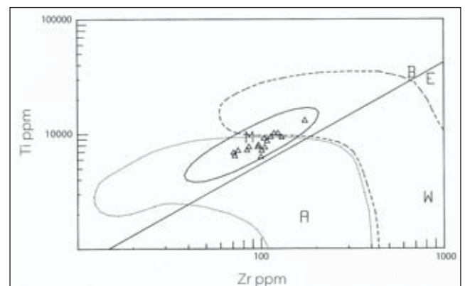
Fig. 32. Plot of \log \text{Ti}/\log \text{Zr} . Fields after Pearce (1982); B = basaltic compositions, E = evolved compositions, M = mid-ocean ridge basalts, A = arc lavas, W = within-plate lavas.
