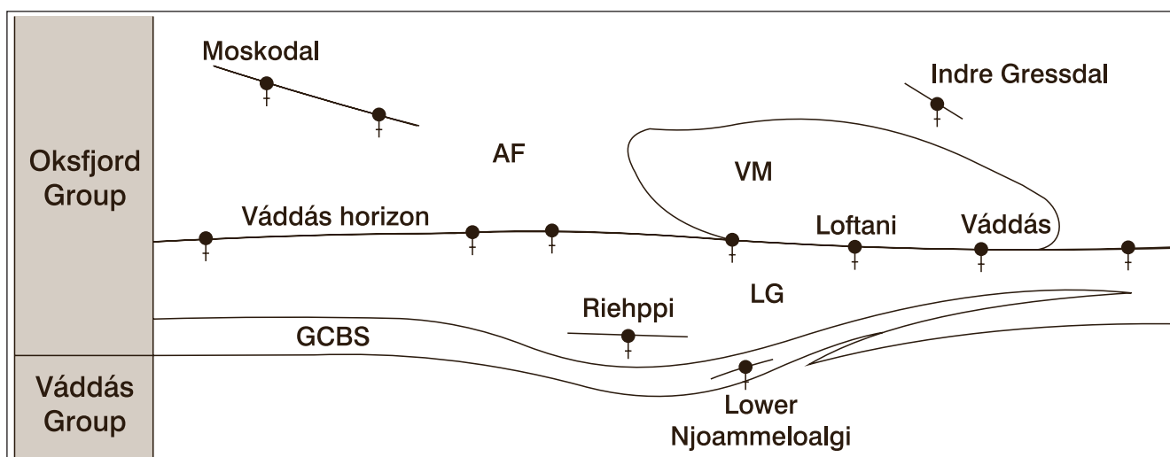
Fig. 12. Schematic locations of the sulphide mineralisations in the Váddás area. GCBS – Goddejávri Calc-Biotite Schist Member; LG – Loftani Greenstone Member; AF – Ankerlia Formation; VM – Váddásgáissá Metagabbro.
