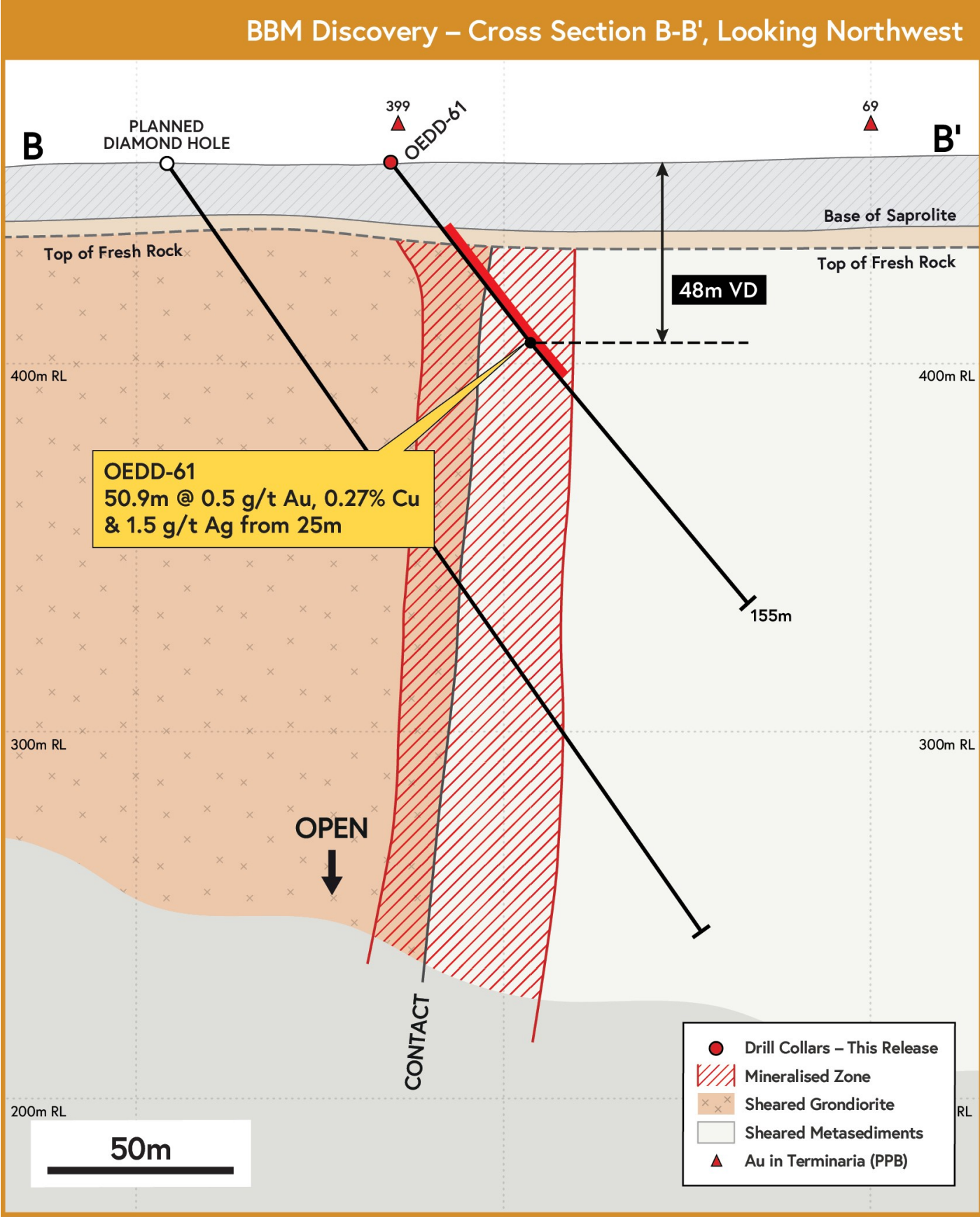
Figure 4: BBM drill section B-B'.
